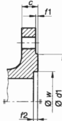
Type G: O-ring spigot
