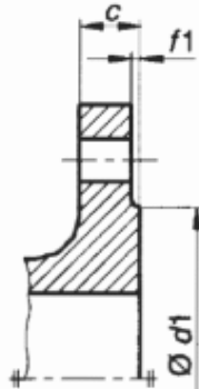
Type B: Raised face (B1 and B2)
