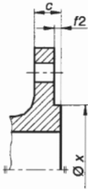
Type E: Spigot
