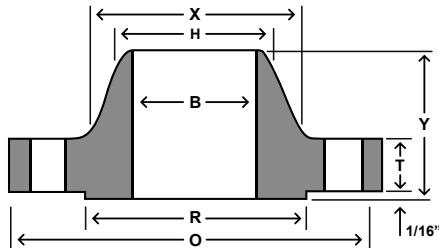
WELD NECK
